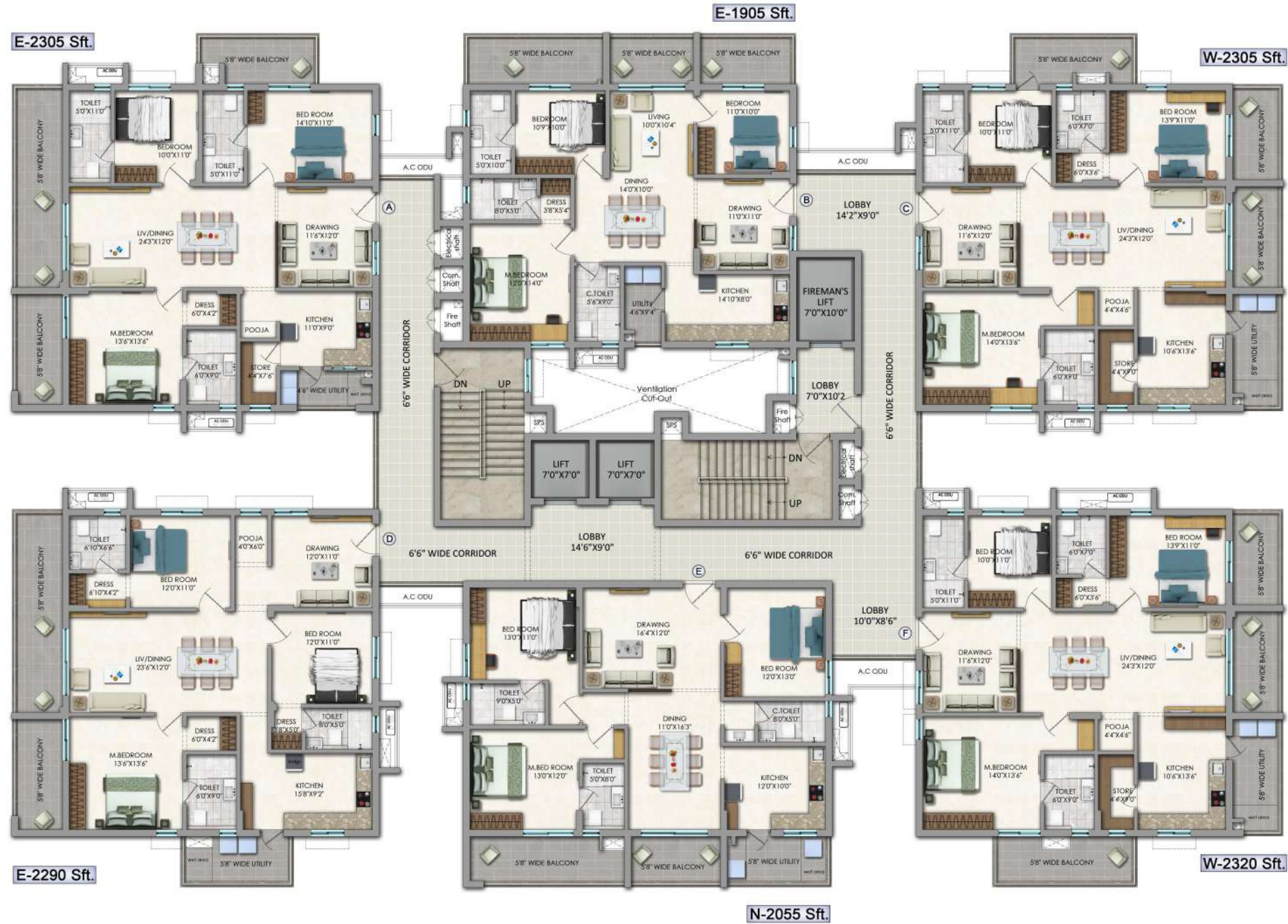
Typical Floor Plan - C
